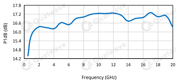
P1dB vs. Frequency
