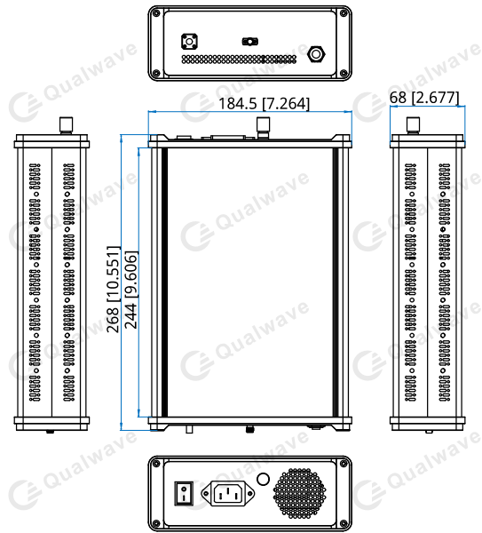
Outline D: Enclosure 0-000006
